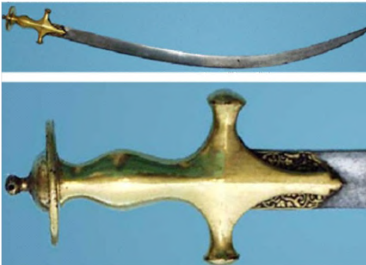
A typical sword made of wootz steel (about 18 th century); the hilt is of iron and coated with a thick layer of gold. (Courtesy: R. Balasubramaniam)
